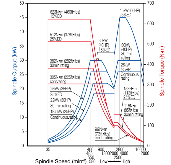
12000min -1 [45/30/26kW(60/40/35HP) MS]
