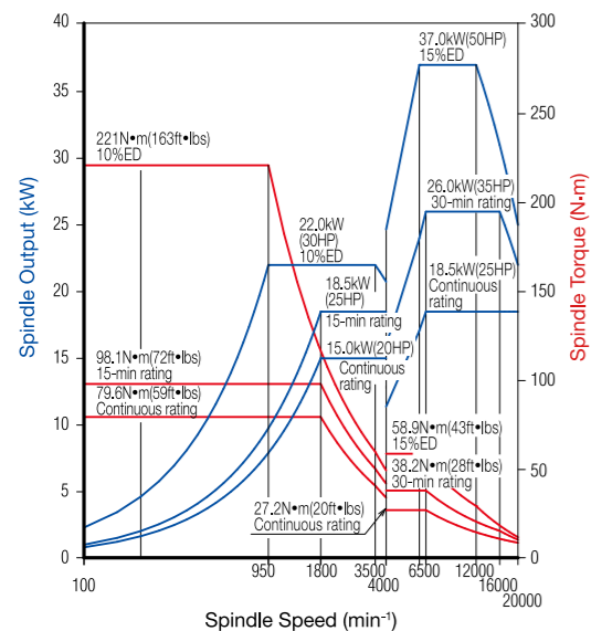
20000min -1 [37/26/18.5kW(50/35/25HP) MS]
