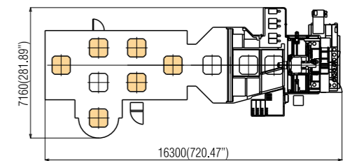
[6-pallet vertical type with set-up station]
