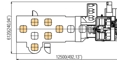
[6-pallet vertical type with set-up station]
