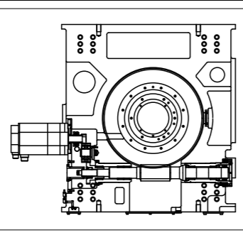
Worm and worm wheel drive (HM800/HM1000S, HM1000/HM1250S)
