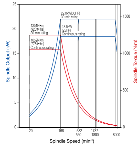
8000min -1 [22 / 18.5kW(30/25HP) Gear]
