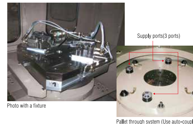
Pallet through system (Use auto-coupler)
